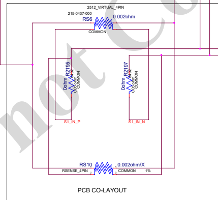
RSENSE2 in Parallel
